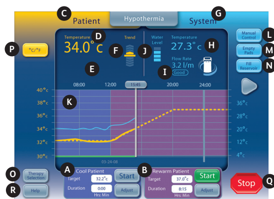
Afb. 1-5 Therapiescherm Hypothermie
